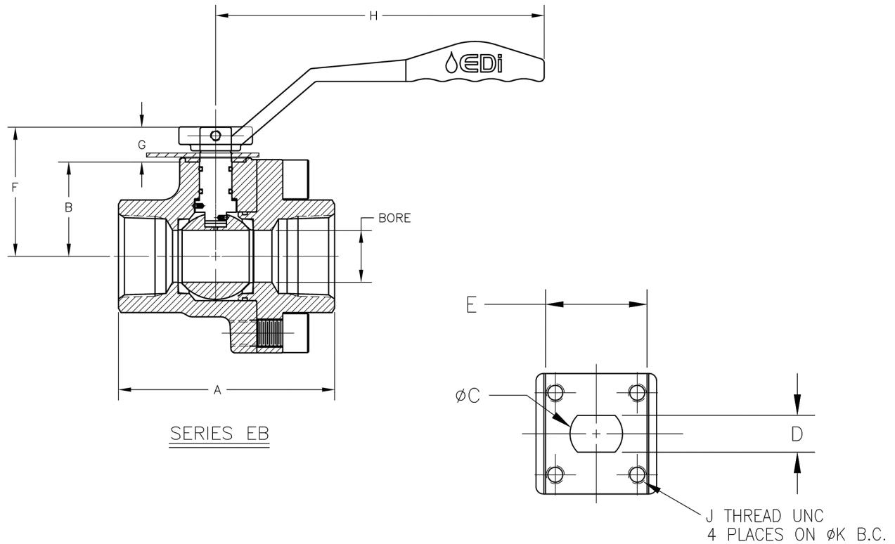
ACTUATOR MOUNTING DETAIL
